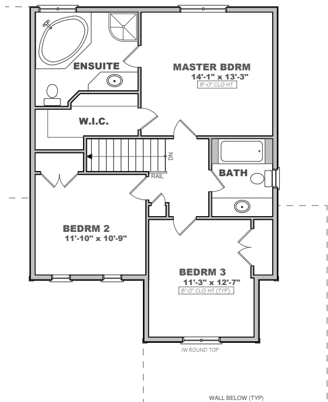
2ND FLOOR PLAN 863 sq ft
