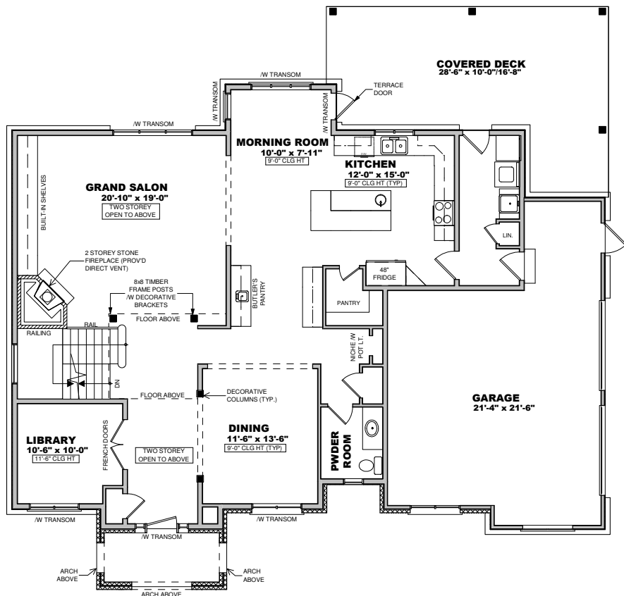
MAIN FLOOR PLAN 1,765 sq ft
