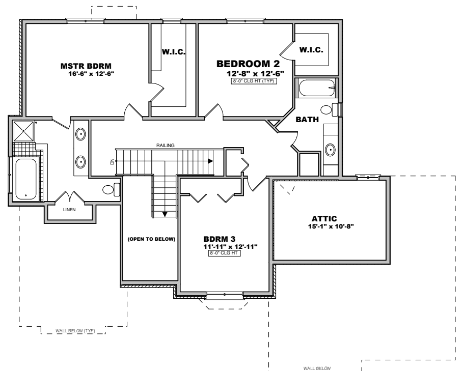
2ND FLOOR PLAN 1,183 sq ft
