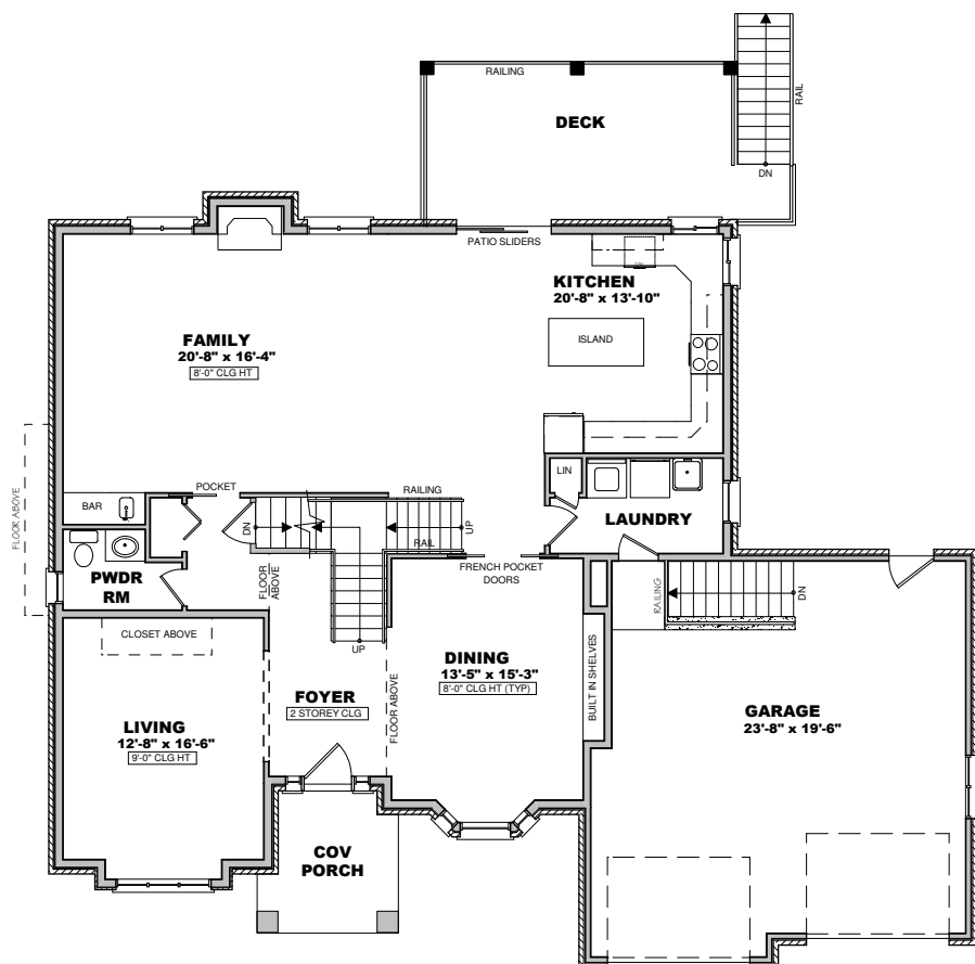
MAIN FLOOR PLAN 1,575 sq ft
