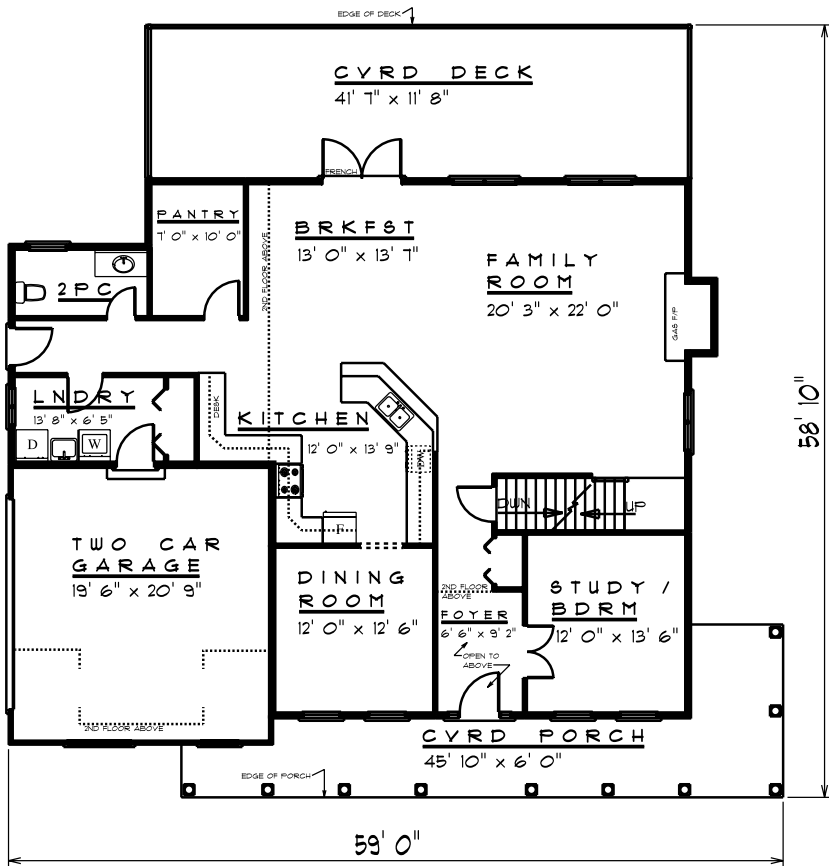
MAIN FLOOR PLAN 1,722 sq ft
